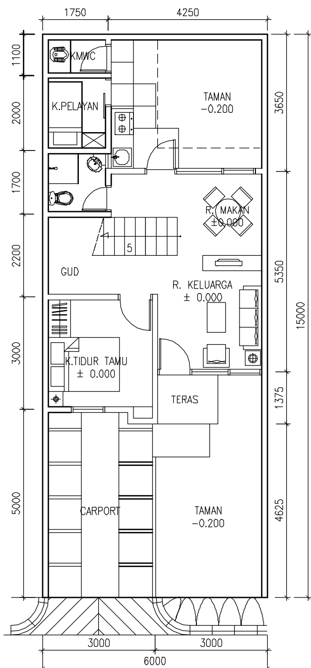
— — DENAH LT.BAWAH TYPE 84/90 SCALE 1 : 50
